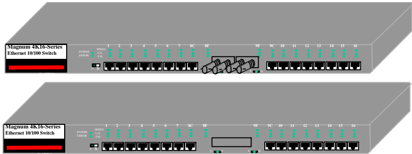
Figure 2.2.1a: Front view, 16-port Magnum 4K16 Series Switches
